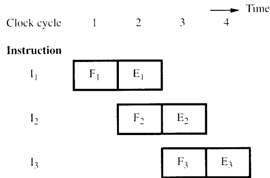
(c) Pipelined execution
