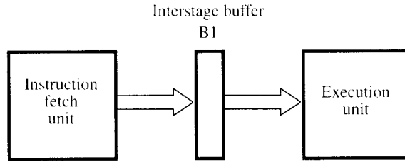
(b) Hardware organization
