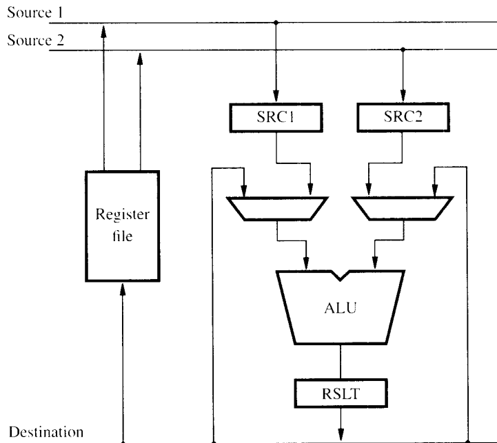
(a) Datapath
