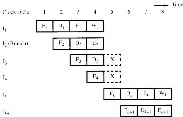
(a) Branch address computed in Execute stage
