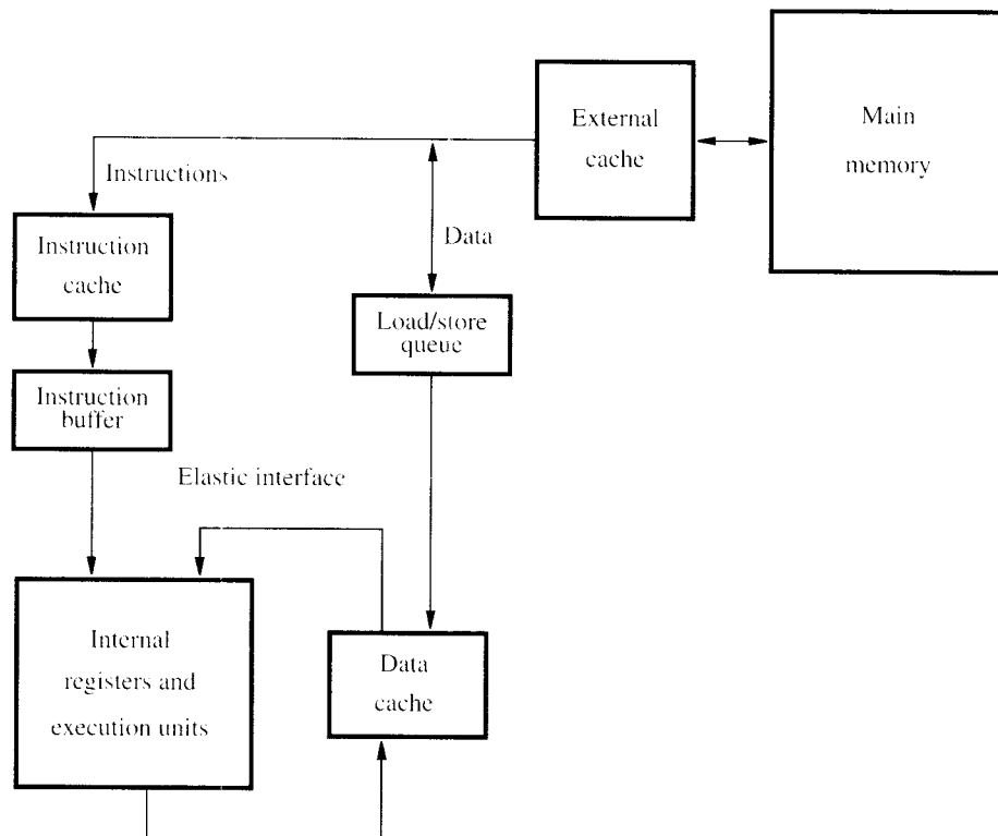
Figure 8.30 Execution flow.
